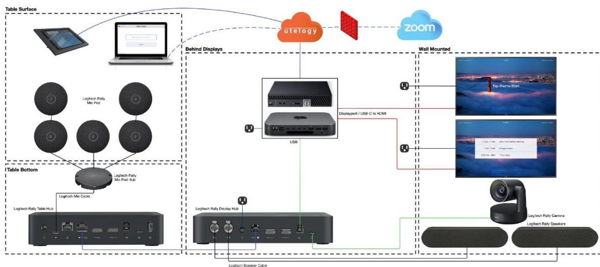
Pictorial Diagram of a Zoom Room Using Utelogy and Logitech Rally
